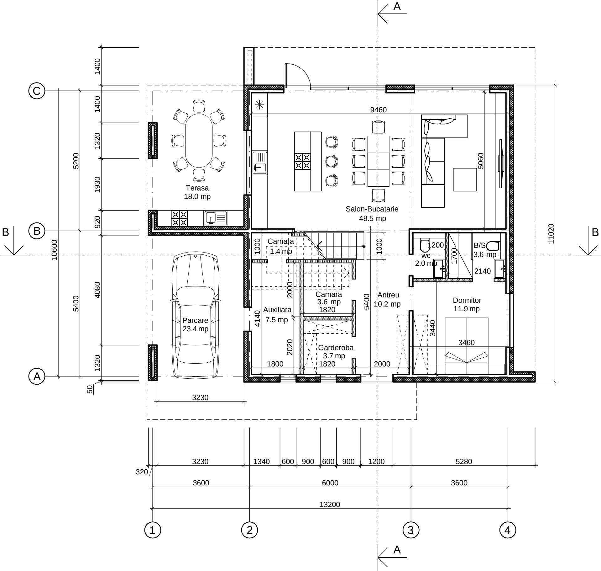
Plan parter Cota 0.000, Sc 1:100 92.4 mp
